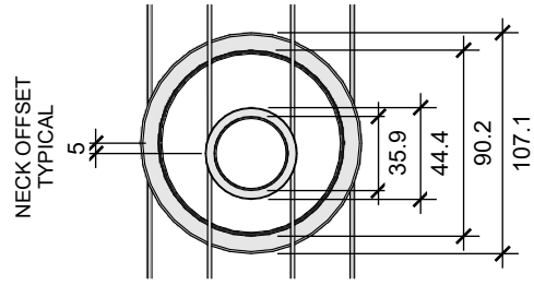
RING DETAIL 1:4
