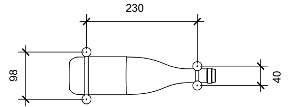
TOP VIEW 1:8
